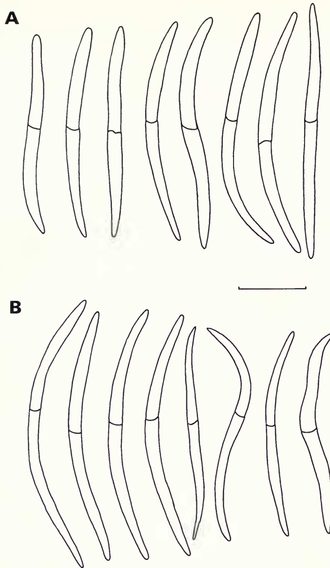
Fig. 11 Ascospore outlines (A) Leptorhaphis laricis (Lahm) Aguirre (PC-HUE 3505/4); (B) Leptorhaphis maggiana (Massal.) Körber (BM-lectotype); scale = 10 \mu m.
